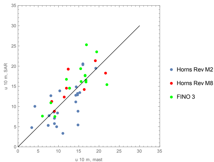
Figure 10: Comparison of wind speed at 10 m, from masts at M2, M8 and FINO3 corrected from other levels to 10 m, and all SAR data at the corresponding pixel cells
